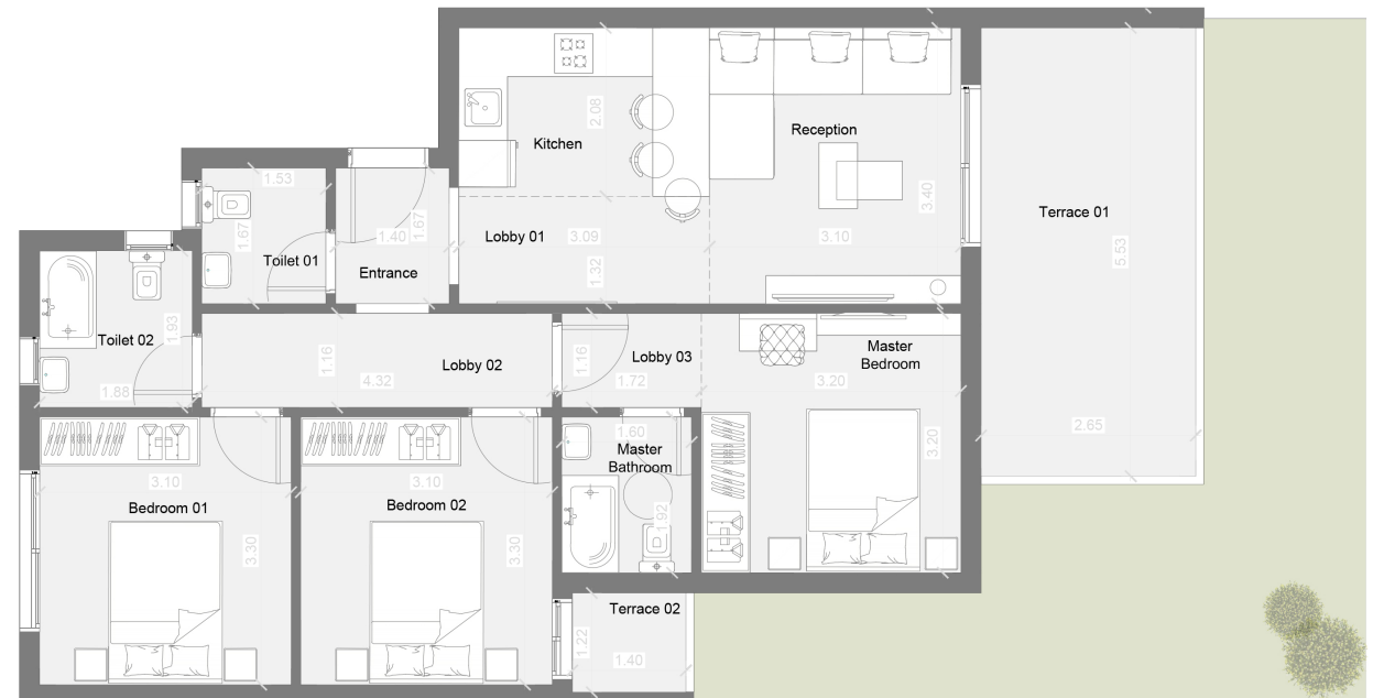
GROUND FLOOR
