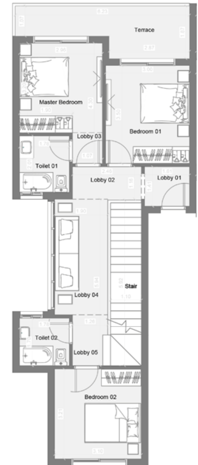
THIRDFLOOR
