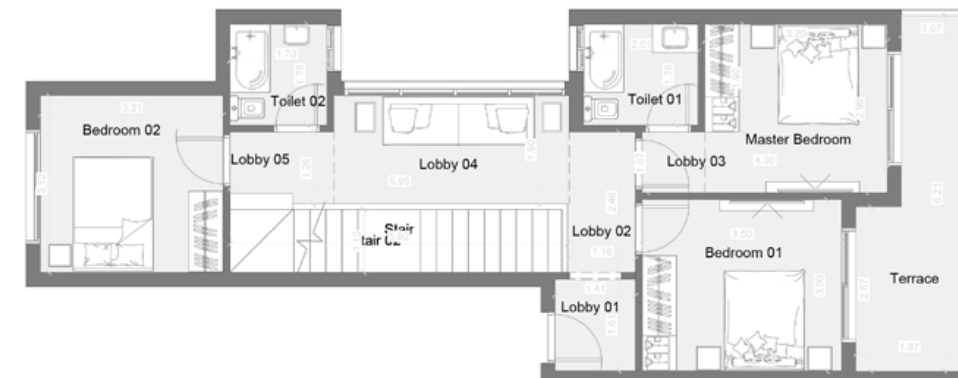
THIRD FLOOR
