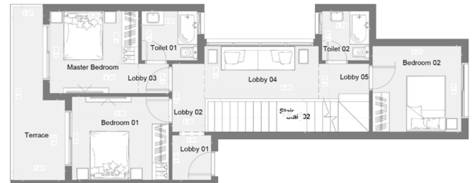
THIRD FLOOR
