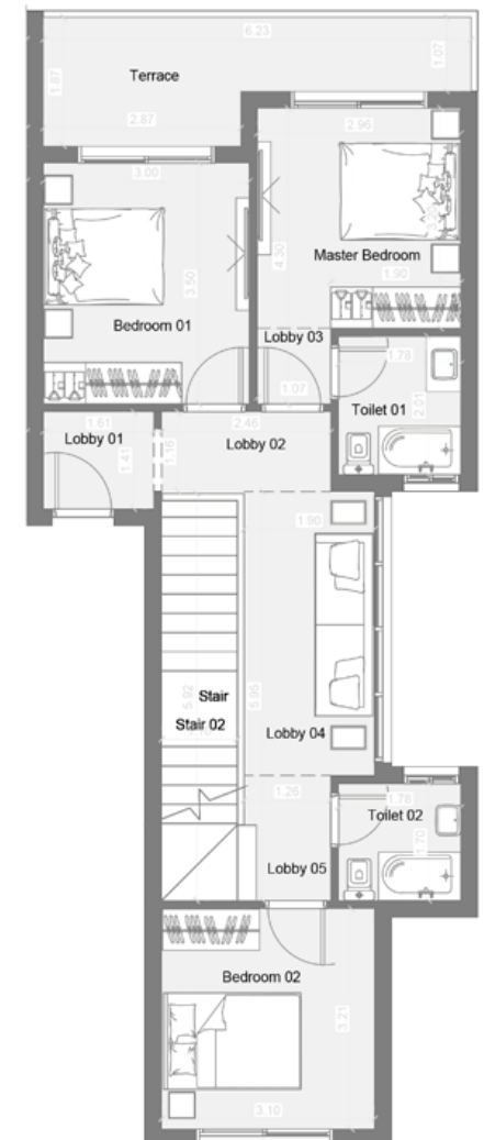
THIRDFLOOR
