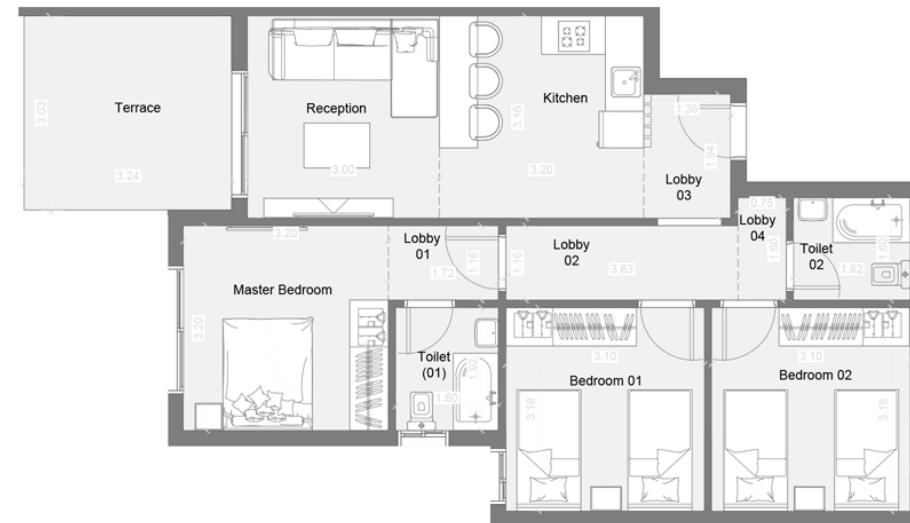
TYPICAL FLOOR
